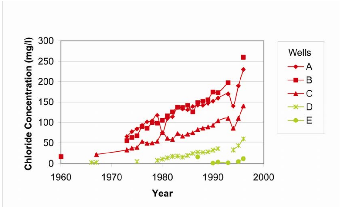
Figure 3. Chloride levels in selected groundwater wells in the Regional Municipality of Waterloo. Red indicates wells from an urbanized area/well field. Green indicates wells from a more rural area/well field. Source: Stanley Consulting (1998)
