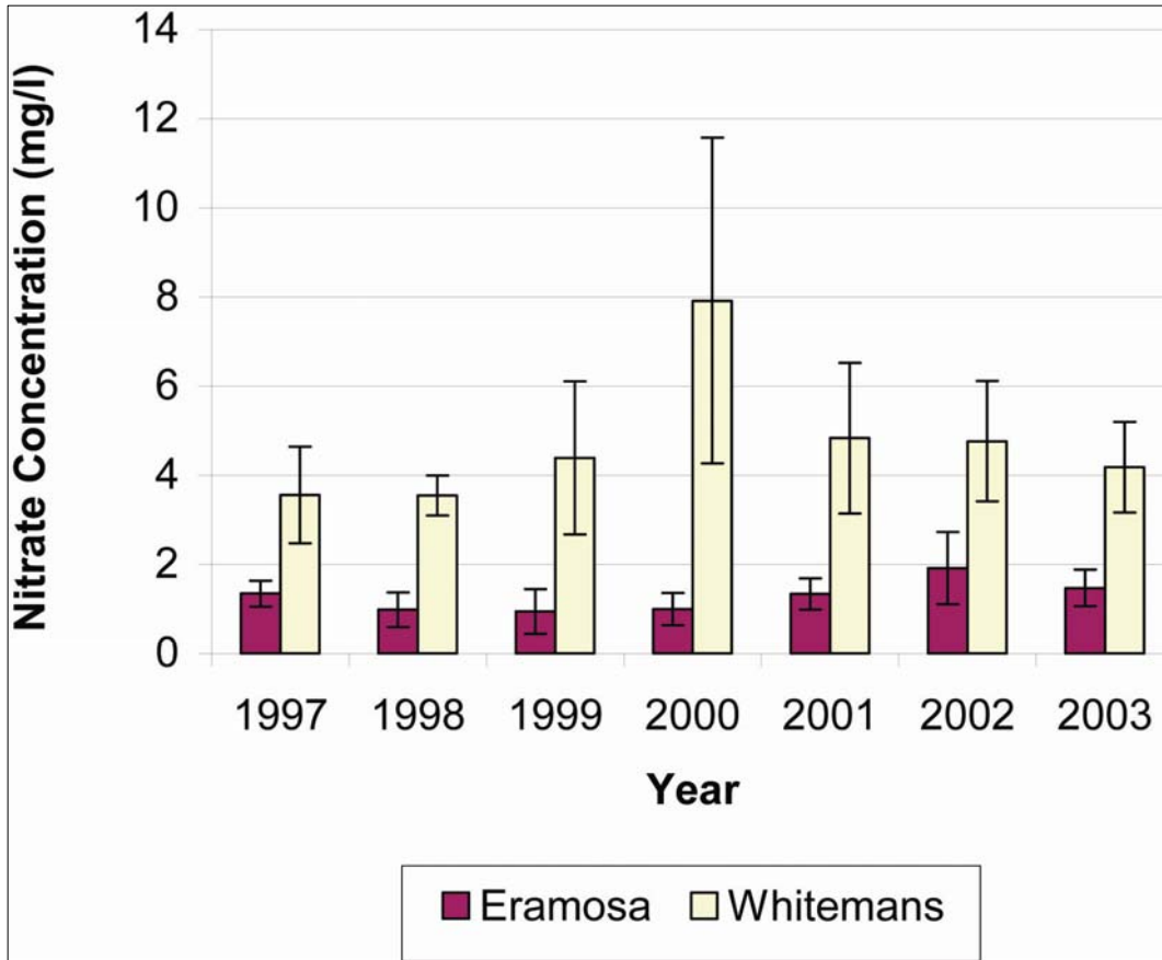
Figure 5. Average annual concentrations of nitrate measured in the Eramosa River and Whitemans Creek from 1997 to 2003. (Also shown on the bar graphs is the standard error of measurement.) Source: Ontario Provincial Water Quality Monitoring Network (2003)
