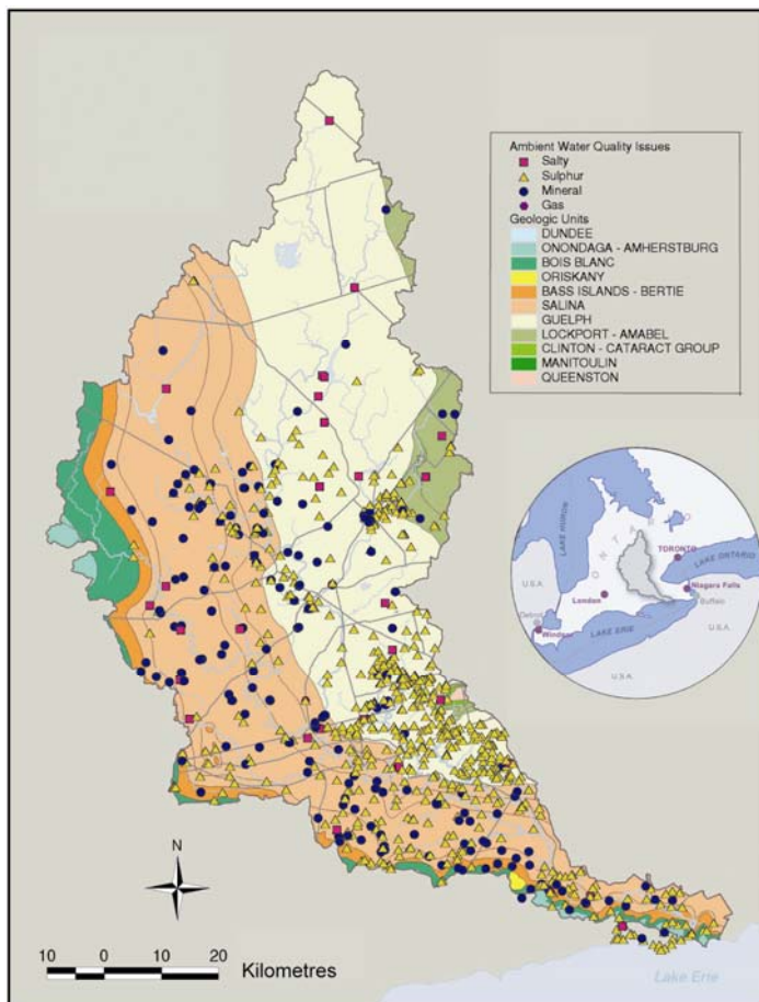
Figure 1. Bedrock wells with natural groundwater quality issues in the Grand River watershed.
